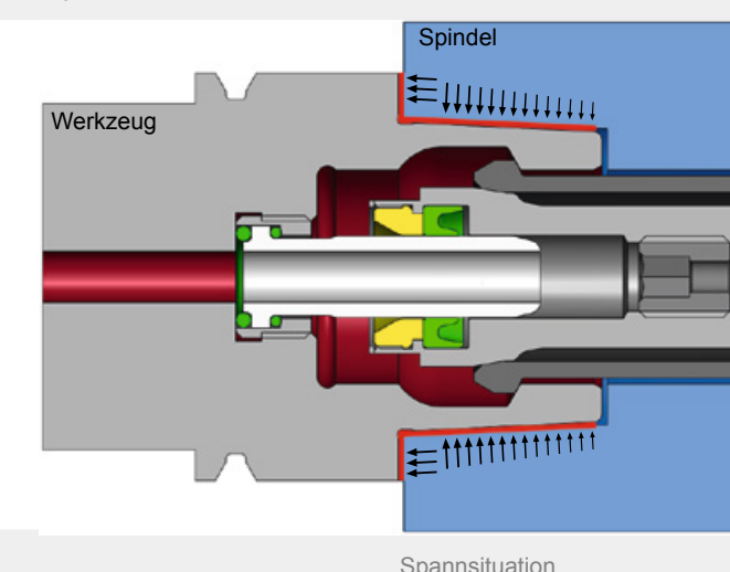
Spannsituation
